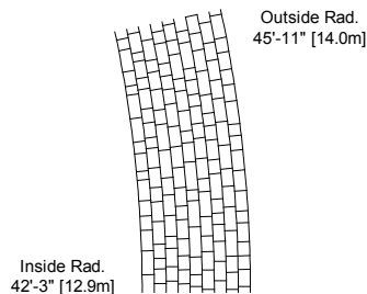
12 ° Section
